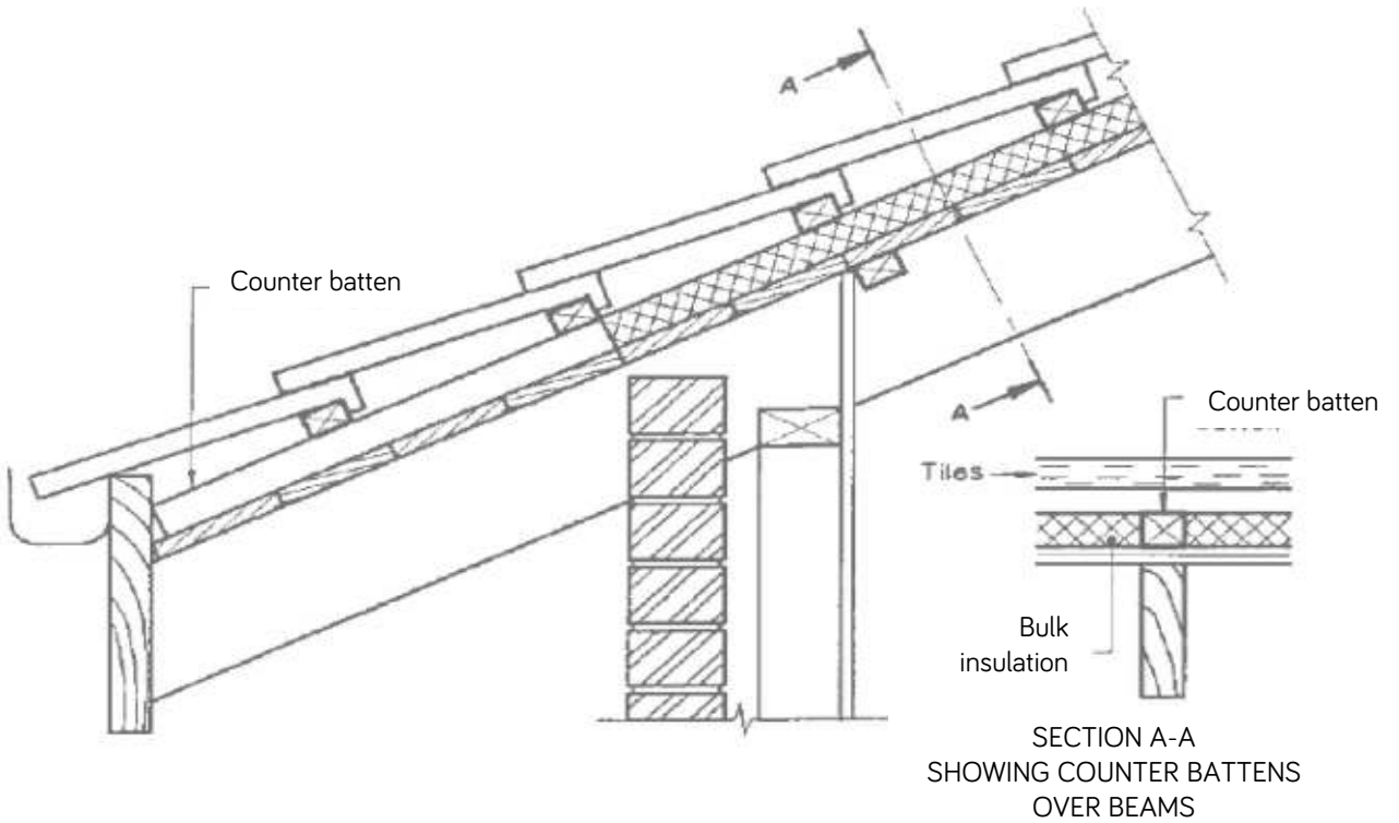
Illustration 13: Bulk Insulation between counter battens / Insulation of sloping ceiling with pitched tiled roofs.
