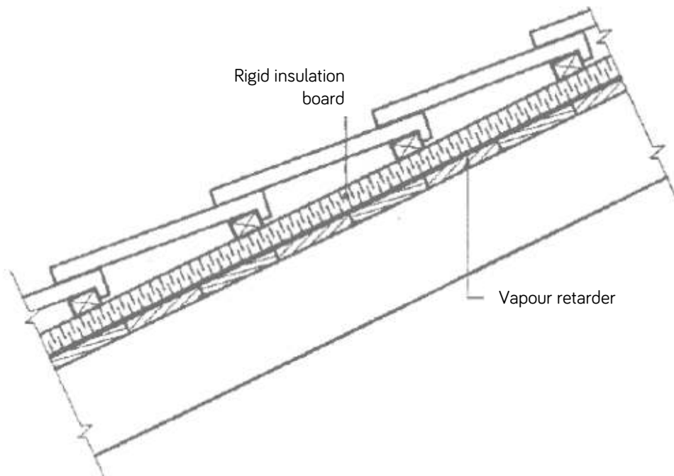
Illustration 14: Rigid board insulation directly over ceiling lining / Insulation of sloping ceiling with pitched, tiles roofs.
