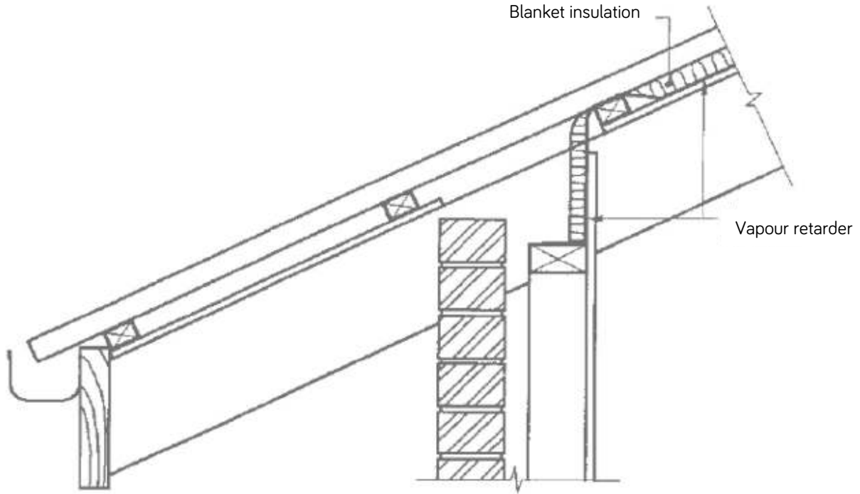
Illustration 15: Insulation of sloping ceiling with pitched, metal roof and exposed beams.
