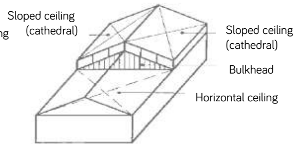
(b) Split level construction
