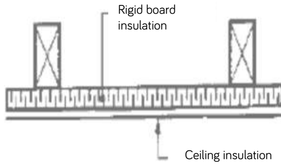
Illustration 7: Rigid board installed between ceiling joists and lining
