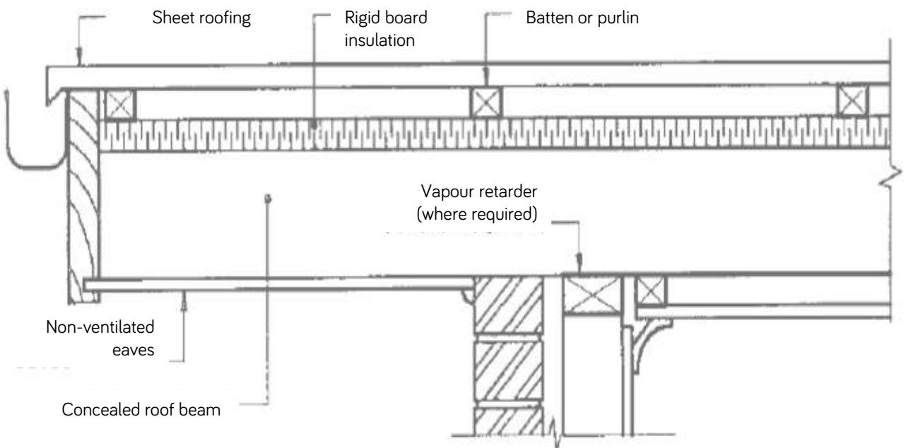
Illustration 10: Rigid board insulation beneath roofing battens.
