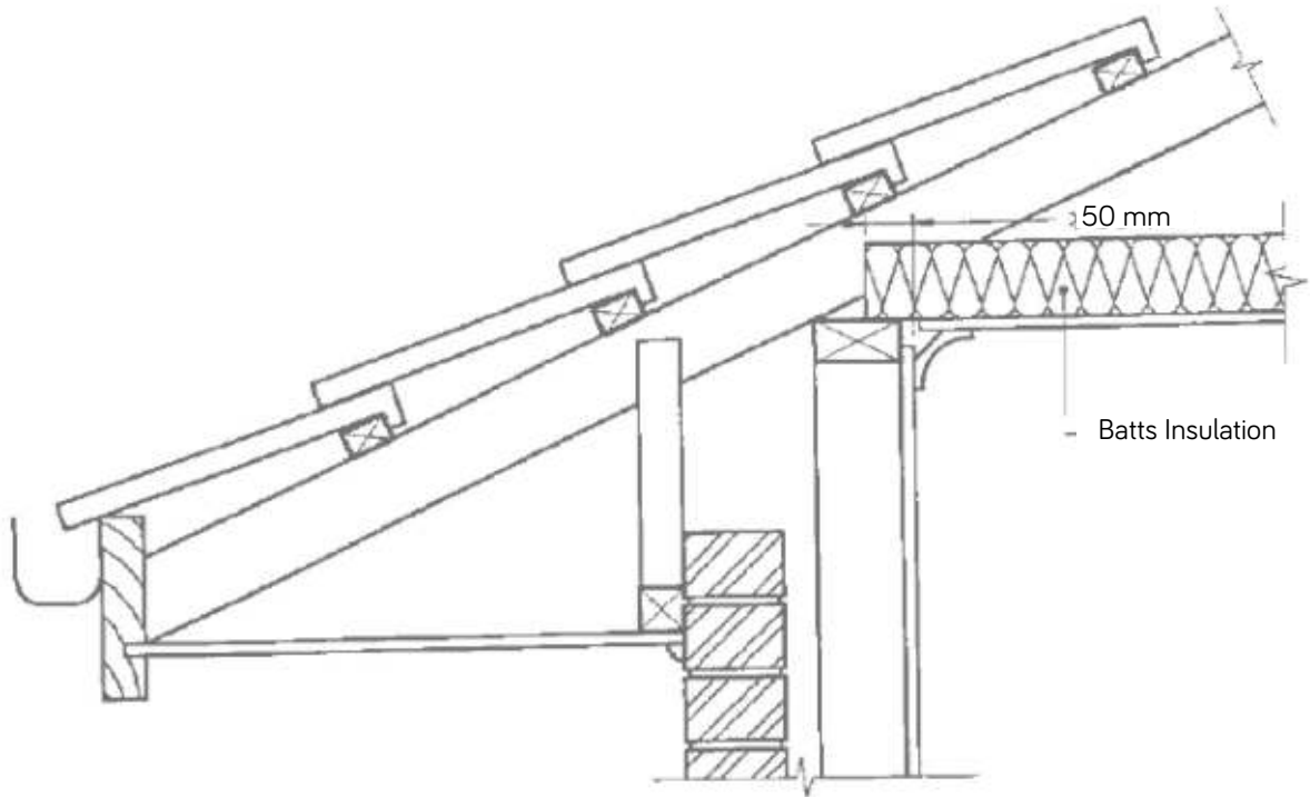
Illustration 3: Extension of ceiling insulation beyond inside face of wall.
