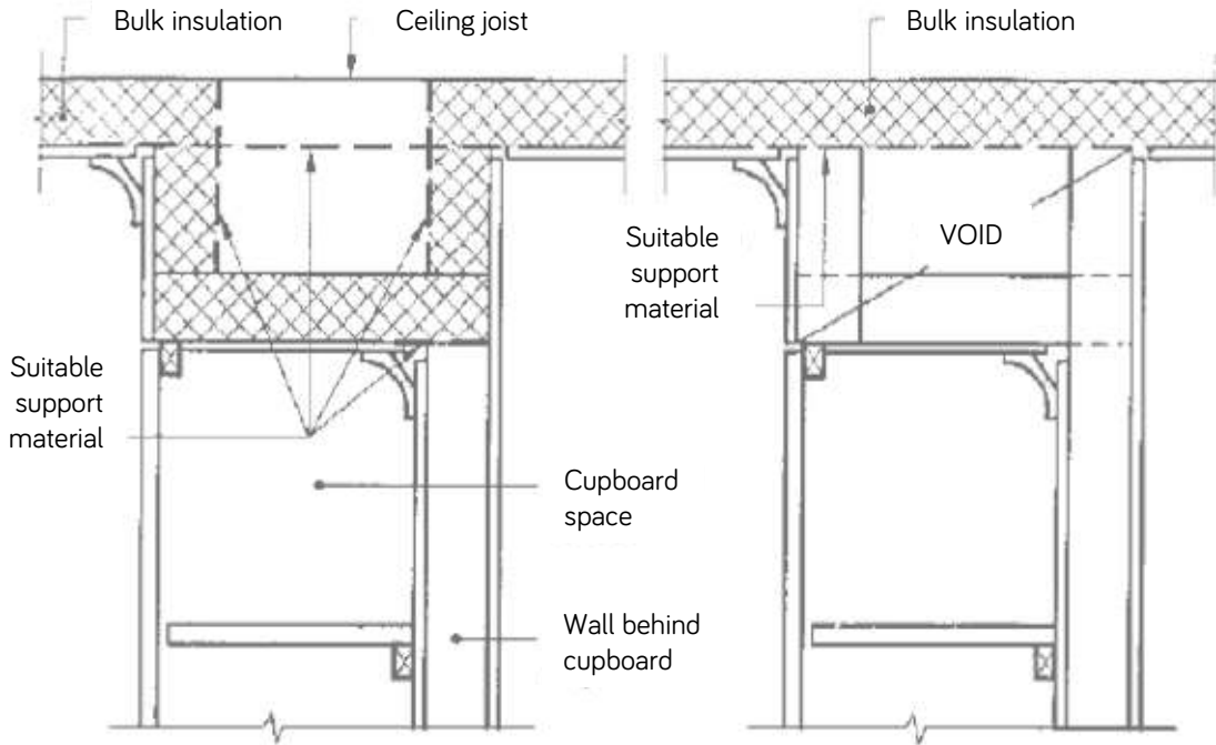
Illustration 5: Alternative treatments for drop ceilings or cavities below ceiling line.
