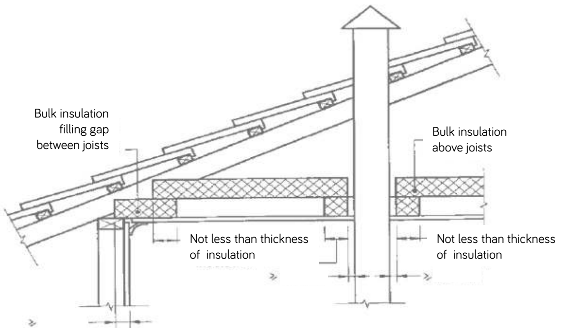
Illustration 4: Prevention of air flow below insulation installed on top of ceiling joists.
