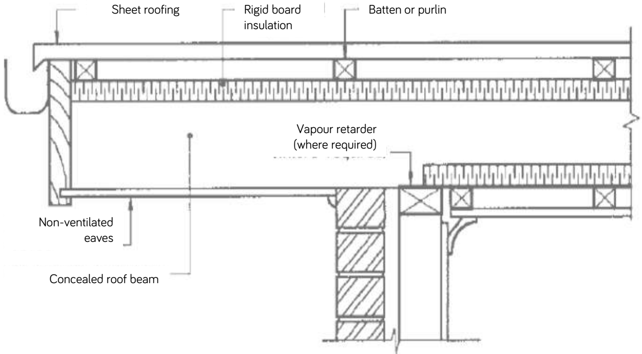
Illustration 11: Rigid board insulation beneath battens and on ceiling / Insulation of horizontal ceilings with flat or low pitched metal roofs.
