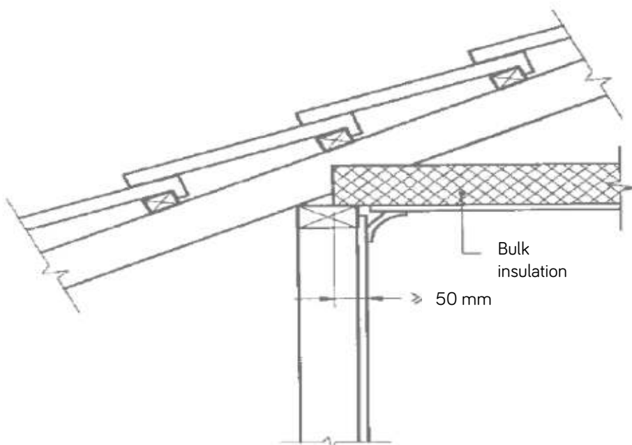
Illustration 12: Insulation of horizontal ceiling with pitched tiled roofs.
