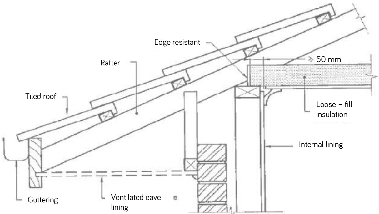
Illustration 1: Placement of thermal insulation to eliminate thermal bridging.
