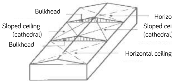
(c) Terrace construction
