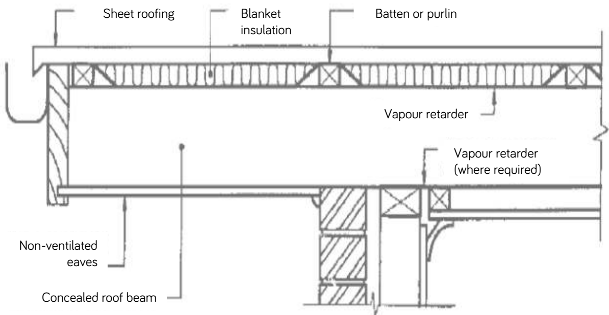
Illustration 8: Blanket insulation in contact with roof sheeting.
