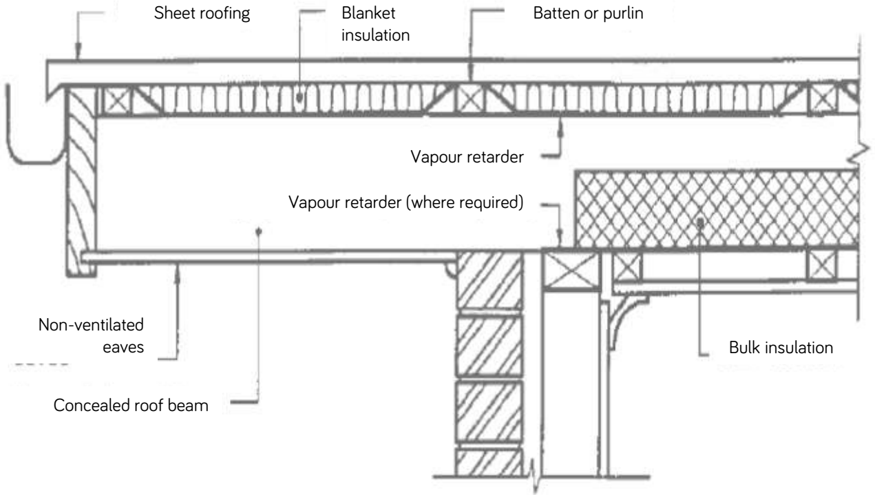
Illustration 9: Blanket insulation in contact with sheet roofing and bulk insulation on ceiling & Insulation of horizontal ceilings with flat or low pitched metal roofs
